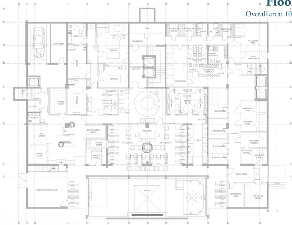
SPA center, technical rooms, restaurant kitchen, stairs, elevators
